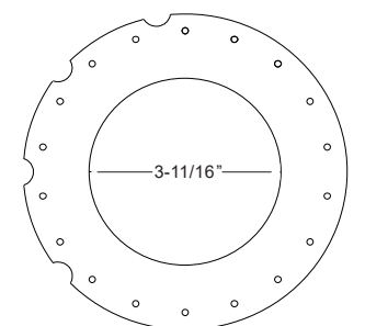
Extra Large Baffle (4 notches) Cup Rim Diameters: 4 1/4" - 4 1/2" Approx. Cup Sizes: 32 - 44 oz. Part: SLRB-2XL
